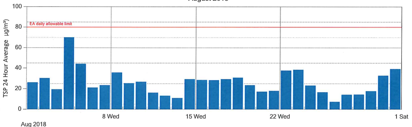
Figure 1: Jondaryan Township TSP continuous monitoring 24 Hr average results for August 2018
