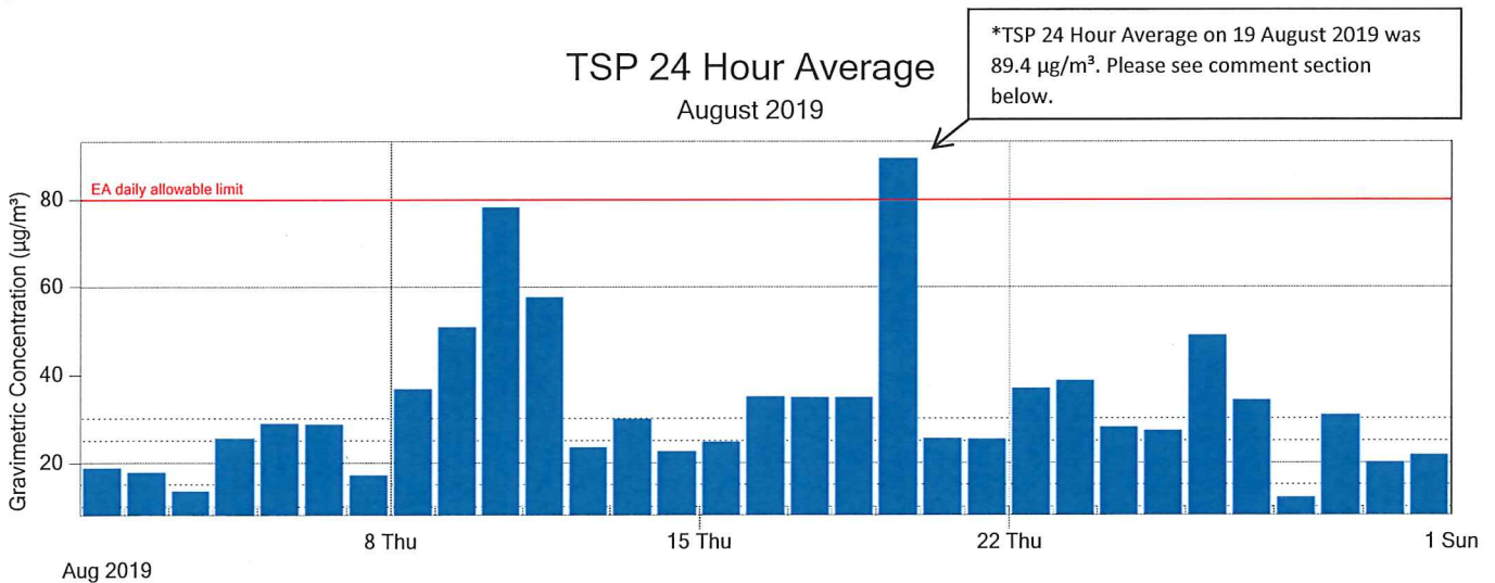
Figure 1: Jondaryan Township TSP continuous monitoring 24 Hr average results for August 2019
