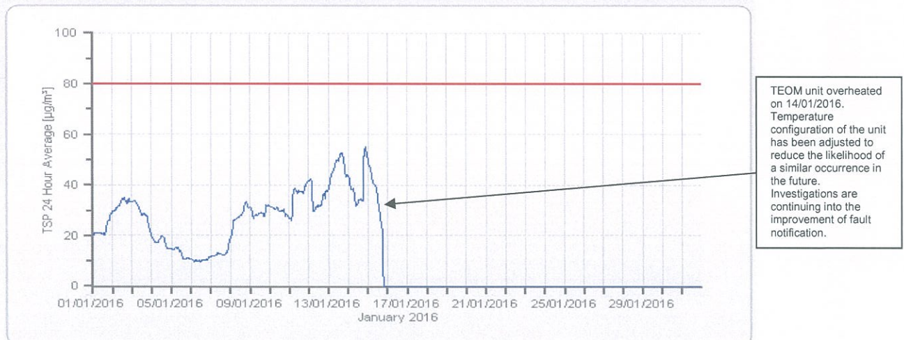
Figure 1: Jondaryan Township TSP continuous monitoring results for the period: January 2016
