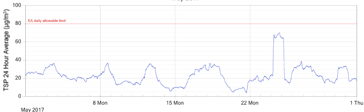
Figure 1: Jondaryan Township TSP continuous monitoring results for May 2017
