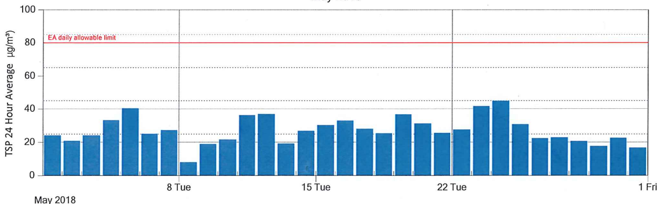
Figure 1: Jondaryan Township TSP continuous monitoring 24 Hr average results for May 2018
