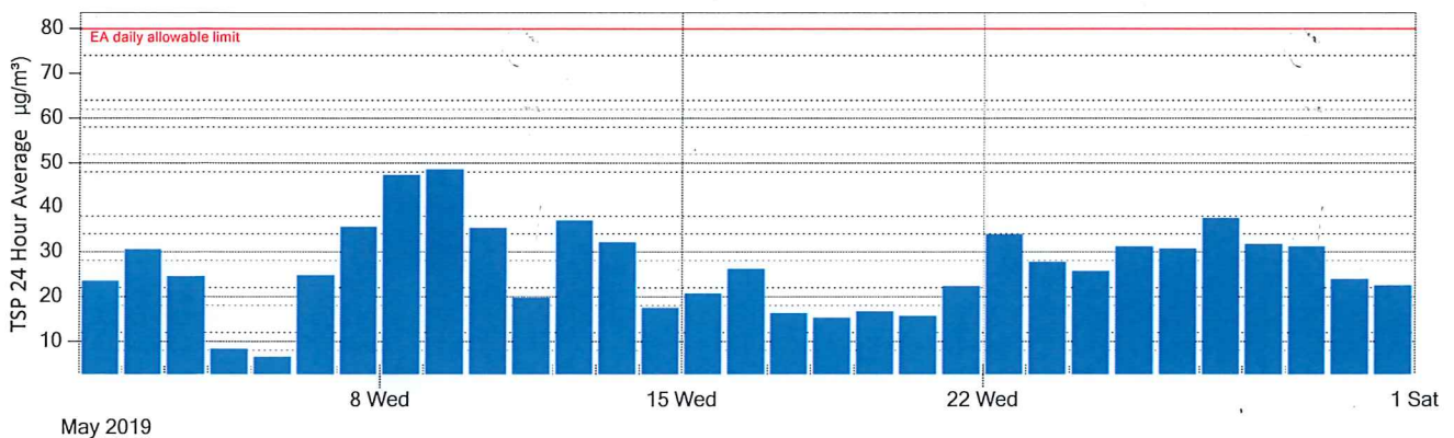
Figure 1: Jondaryan Township TSP continuous monitoring 24 Hr average results for May 2019
