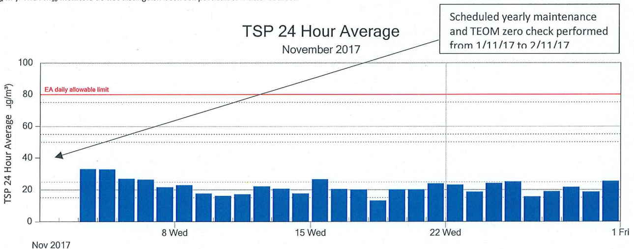
Figure 1: Jondaryan Township TSP continuous monitoring 24 Hr average results for November 2017
