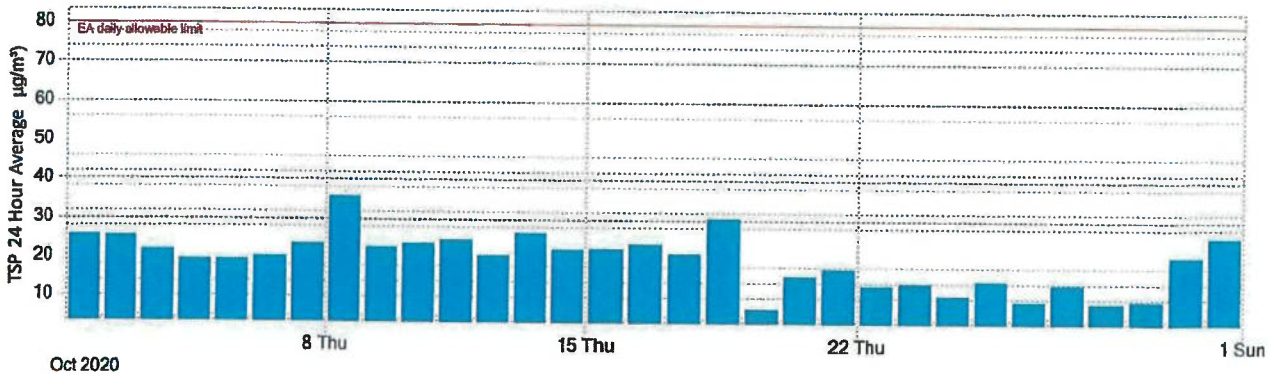
Figure 1: Jondaryan Township TSP continuous monitoring 24 Hr average results for October 2020
